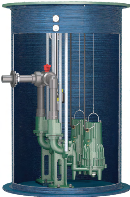
FIBERGLASS & POLYETHYLENE BASINS, PRE-FABRICATED LIFT STATIONS.
